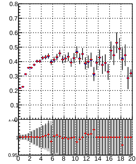
Fake rate vs. \bullet DQM_TT_mkFit-DQM_init_orig \bullet DQM_TT_mkFit-DQM_init_mod2
