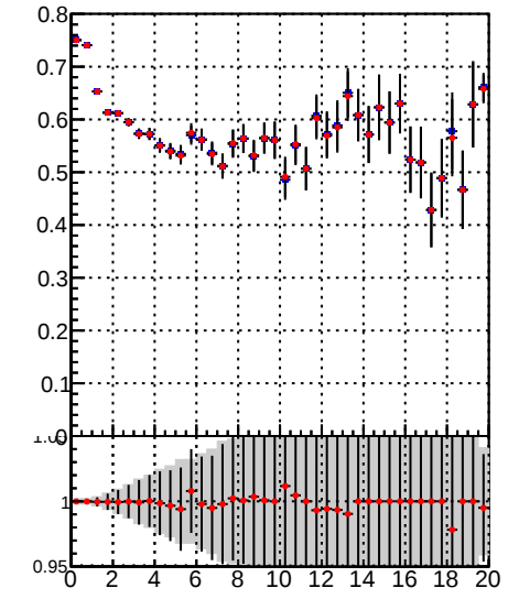
Fake rate vs. \bullet DQM_TT_mkFit-DQM_init_orig \bullet DQM_TT_mkFit-DQM_init_mod2
