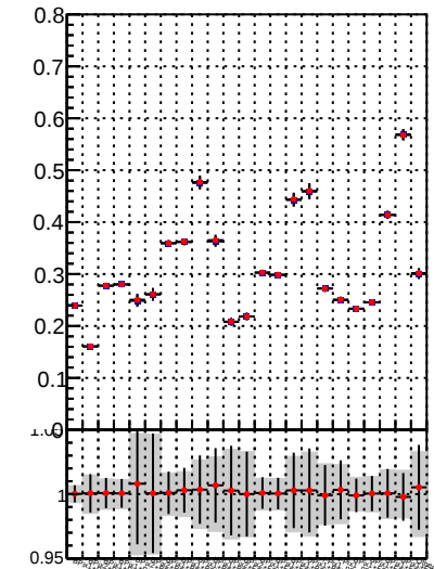
Fake rate vs. \bullet DQM_TT_mkFit-DQM_init_orig \bullet DQM_TT_mkFit-DQM_init_mod2
