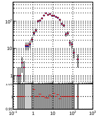
—●— DQM_TT_mkFit-DQM_init_orig —●— DQM_TT_mkFit-DQM_init_modi2
