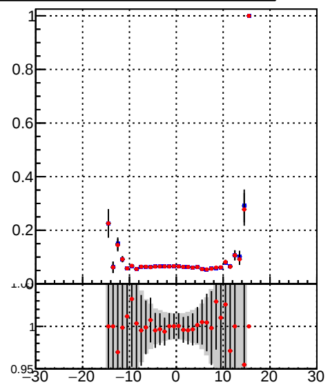
Efficiency vs. sim PV z Legend: DQM_TT_mkFit-DQM_init_orig (blue line) DQM_TT_mkFit-DQM_init_modi2 (red line)
