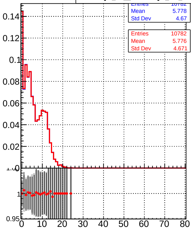
— DQM_TT_mkFit-DQM_init_orig — DQM_TT_mkFit-DQM_init_modi2
