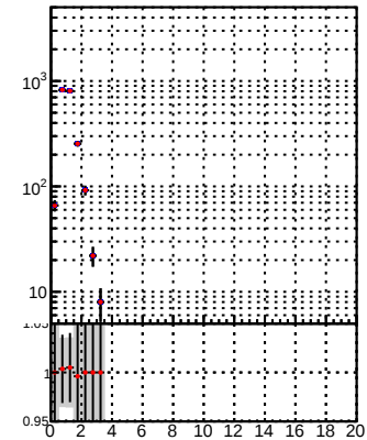
N of reco track vs. \chi^2 for different DQM TT methods
