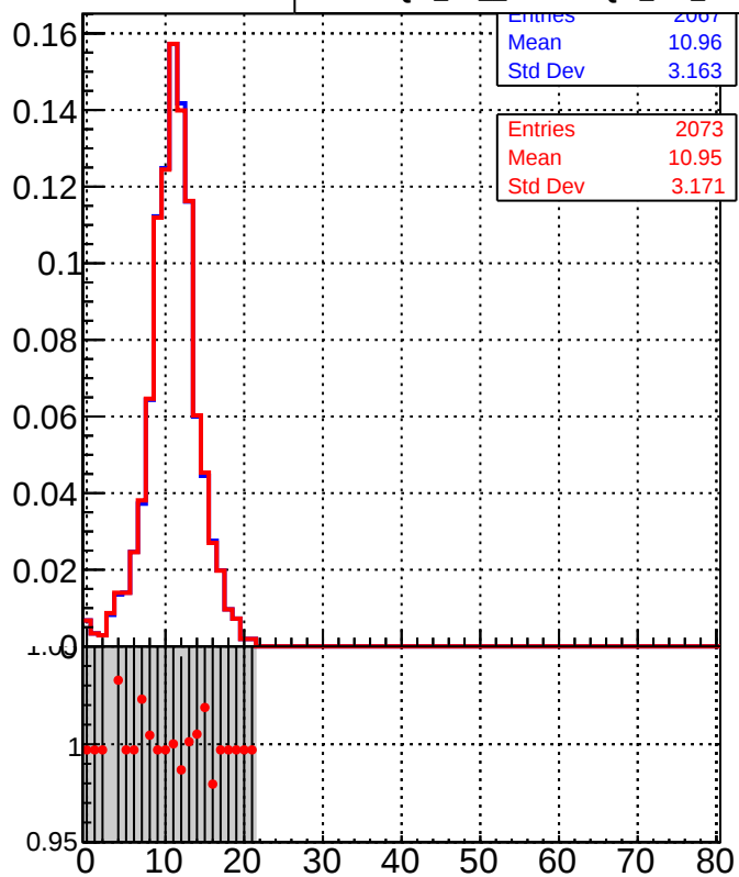
Legend for bottom row plots: ■ DQM_TT_mkFit-DQM_init_orig ● DQM_TT_mkFit-DQM_init_modi2
