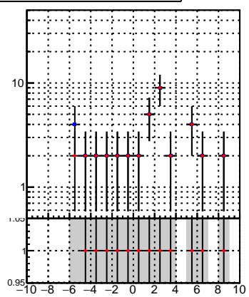
Number of associated (recoToSim) loop tracks vs. sim PV z
