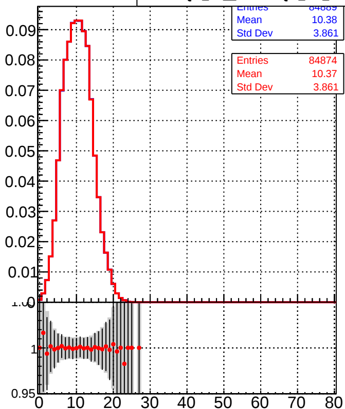
Legend: DQM_TT_mkFit-DQM_init_orig (grey bars) DQM_TT_mkFit-DQM_init_modi2 (red line with markers)
