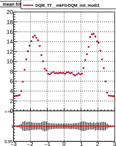
— DQM_TT_mkFit-DQM_init_orig — DQM_TT_mkFit-DQM_init_modi2
