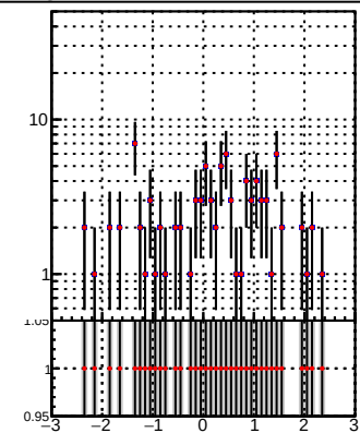
—●— DQM_TT_mkFit-DQM_init_orig —●— DQM_TT_mkFit-DQM_init_modi2
