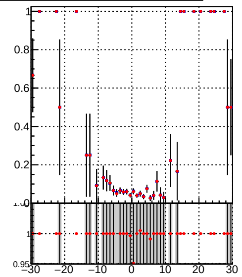
Efficiency vs vertpos — DQM_TT_mkFit-DQM_init_orig — DQM_TT_mkFit-DQM_init_mod2
