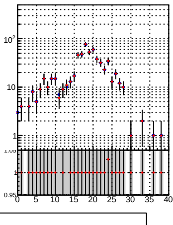
N of associated tracks (simToReco) vs hit
