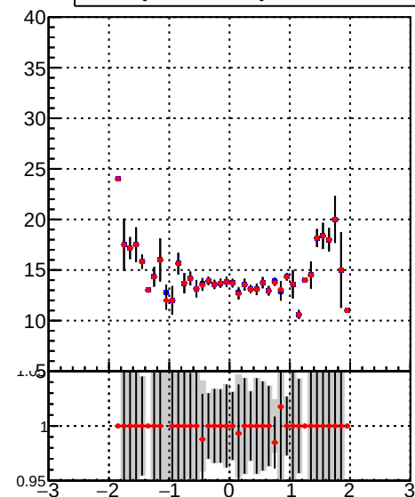
mean hit — DQM_TT_mkFit-DQM_init_orig — DQM_TT_mkFit-DQM_init_mod2
