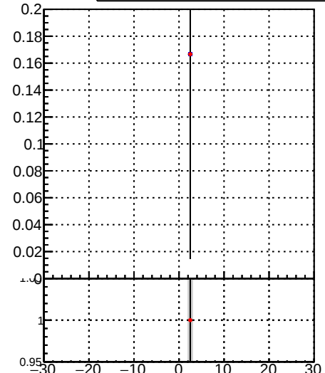
Fake rate vs vertpos DQM_TT_mkFit-DQM_init_orig DQM_TT_mkFit-DQM_init_modi2
