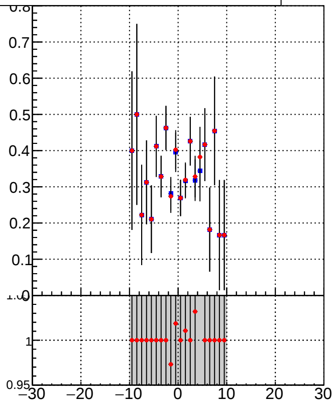
DQM_TT_mkFit-DQM_init_orig DQM_TT_mkFit-DQM_init_modi2
