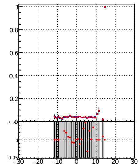
Fake rate vs d DQM_TT_mkFit-DQM_init_orig DQM_TT_mkFit-DQM_init_modi2
