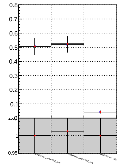
Fake rate vs. DQM_TT_mkFit-DQM_init_orig DQM_TT_mkFit-DQM_init_modi2
