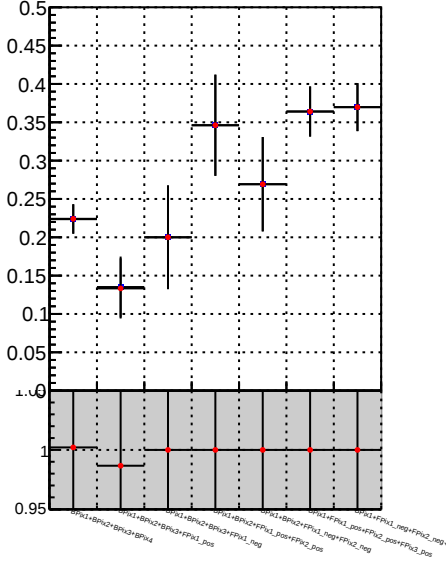
Fake rate vs. \bullet DQM_TT_mkFit-DQM_init_orig \bullet DQM_TT_mkFit-DQM_init_modi2
