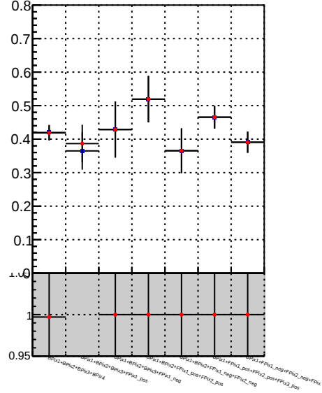
Fake rate vs. \bullet DQM_TT_mkFit-DQM_init_orig \bullet DQM_TT_mkFit-DQM_init_modi2
