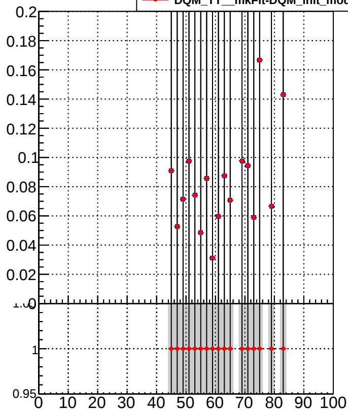
■ DQM_TT_mkFit-DQM_init_orig ● DQM_TT_mkFit-DQM_init_modi2
