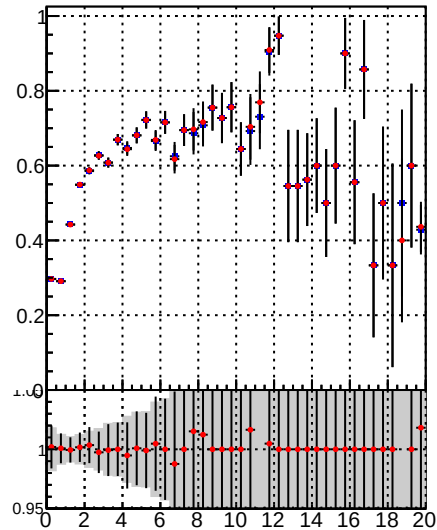
Fake rate vs. \text{DQM\_TT\_mkFit-DQM\_init\_orig} \text{DQM\_TT\_mkFit-DQM\_init\_modi2}
