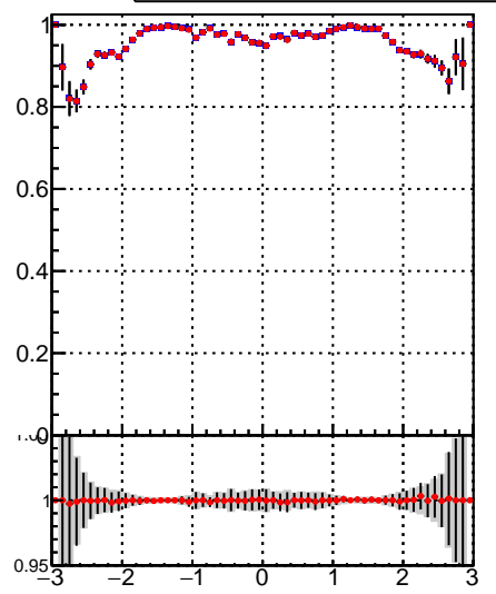
Legend for the middle row of plots: DQM_TT_mkFit-DQM_init_orig (blue squares) DQM_TT_mkFit-DQM_init_modi2 (red circles)
