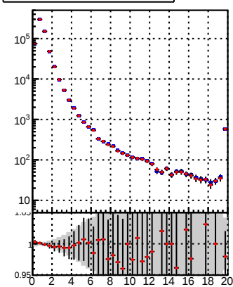
N of assoc (recoToSim) tracks vs normalized \chi^2
