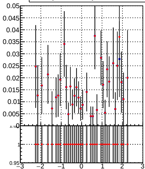
—•— DQM_TT_mkFit-DQM_init_orig —•— DQM_TT_mkFit-DQM_init_modi2
