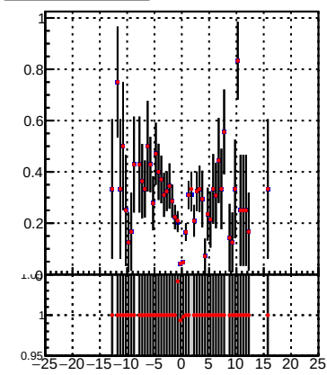
Efficiency vs Dxy(PV) Legend: DQM_TT_mkFit-DQM_init_orig DQM_TT_mkFit-DQM_init_mod2
