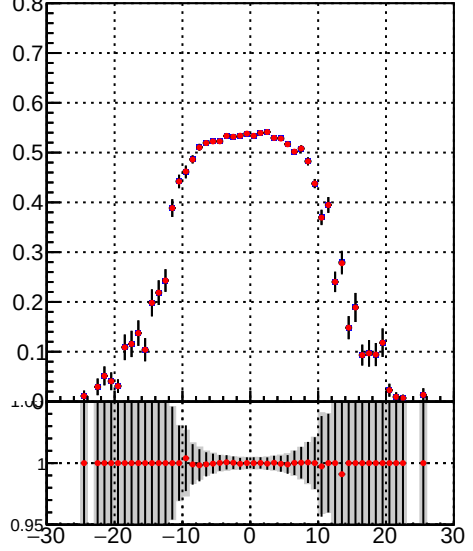
Efficiency vs. sim PV z — DQM_TT_mkFit-DQM_init_orig — DQM_TT_mkFit-DQM_init_mod2
