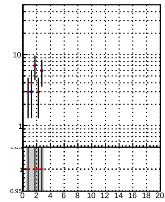
N of reco track vs. \chi^2 for different initialization methods
