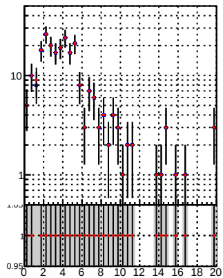
N of reco track vs. \chi^2 for DQM TT mkFit-DQM_init_orig and DQM TT mkFit-DQM_init_modi2
