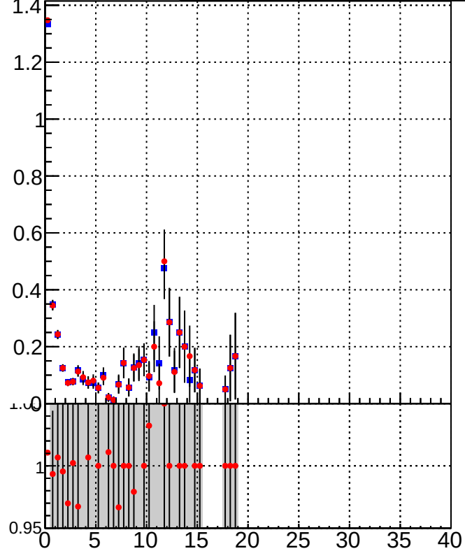
K_S^0 tracking fake rate vs p_T \blacksquare DQM_TT_mkFit-DQM_init_orig \bullet DQM_TT_mkFit-DQM_init_modi2
