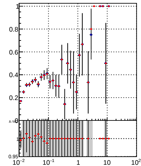
—•— DQM_TT_mkFit-DQM_init_orig —•— DQM_TT_mkFit-DQM_init_modi2
