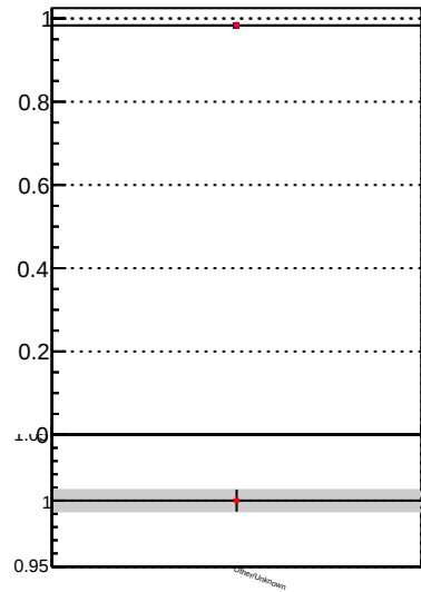
Fake rate vs. —•— DQM_TT_mkFit-DQM_init_orig —•— DQM_TT_mkFit-DQM_init_modi2
