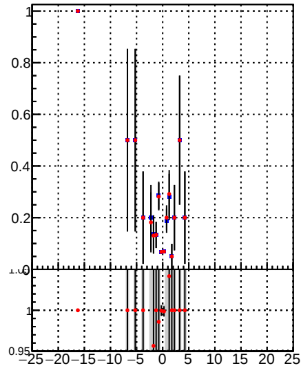
—●— DQM_TT_mkFit-DQM_init_orig —●— DQM_TT_mkFit-DQM_init_modi2
