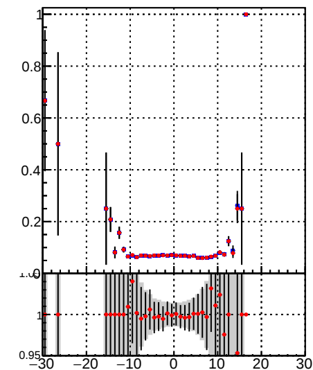
—●— DQM_TT_mkFit-DQM_init_orig —●— DQM_TT_mkFit-DQM_init_modi2
