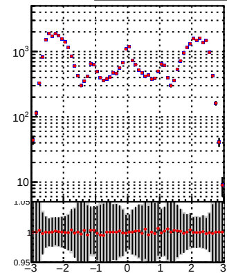
—●— DQM_TT_mkFit-DQM_init_orig —●— DQM_TT_mkFit-DQM_init_modi2
