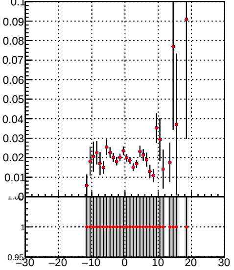
Efficiency vs vertpos —•— DQM_TT_mkFit-DQM_init_orig —•— DQM_TT_mkFit-DQM_init_mod2
