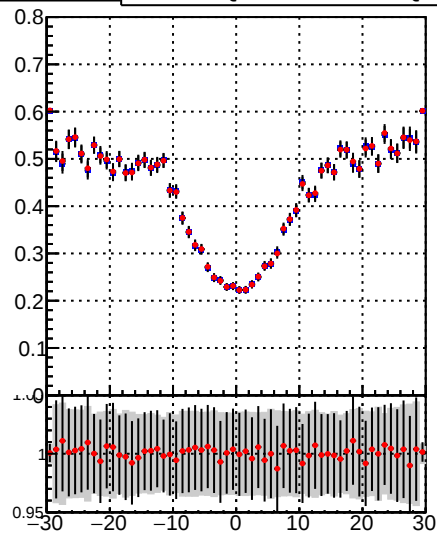
—●— DQM_TT_mkFit-DQM_init_orig —●— DQM_TT_mkFit-DQM_init_modi2
