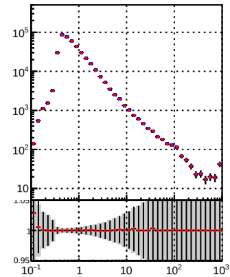
—●— DQM_TT mkFit-DQM_init_orig —●— DQM_TT mkFit-DQM_init_modi2
