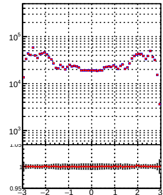
—•— DQM_TT_mkFit-DQM_init_orig —•— DQM_TT_mkFit-DQM_init_modi2
