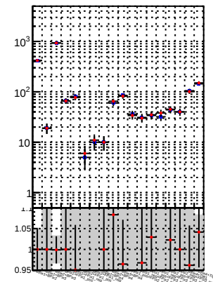
N of reco track vs. \chi^2 —•— DQM TT mkFit-DQM_init_orig —•— DQM TT mkFit-DQM_init_mod12
