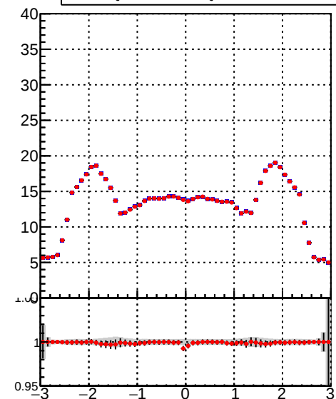
mean hit — DQM_TT_mkFit-DQM_init_orig — DQM_TT_mkFit-DQM_init_modi2
