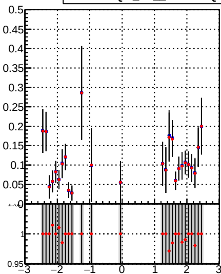
—■— DQM_TT_mkFit-DQM_init_orig —●— DQM_TT_mkFit-DQM_init_modi2
