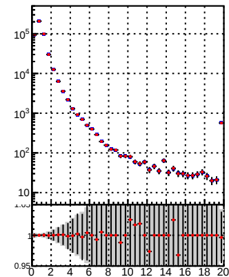
N of orig (recoToSim) tracks vs normalized \chi^2
