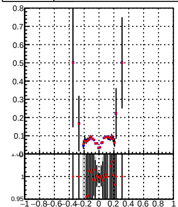
Fake rate vs dzp
