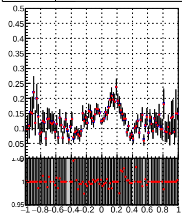
—●— DQM_TT_mkFit-DQM_init_orig —●— DQM_TT_mkFit-DQM_init_modi2
