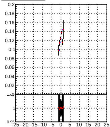
—●— DQM_TT_mkFit-DQM_init_orig —●— DQM_TT_mkFit-DQM_init_modi2
