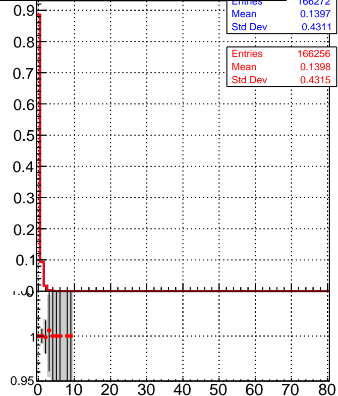
Legend: - DQM_TT_mkFit-DQM_init_orig (grey histogram) - DQM_TT_mkFit-DQM_init_modi2 (red line with markers)
