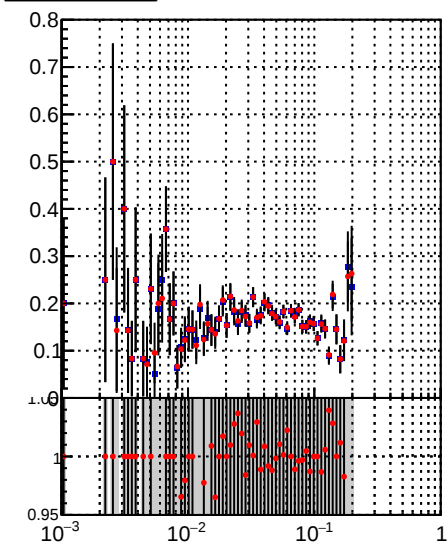
—●— DQM_TT_mkFit-DQM_init_orig —●— DQM_TT_mkFit-DQM_init_modi2
