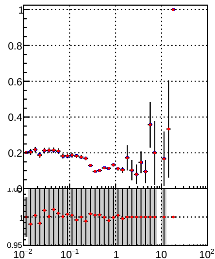
—•— DQM_TT_mkFit-DQM_init_orig —•— DQM_TT_mkFit-DQM_init_modi2
