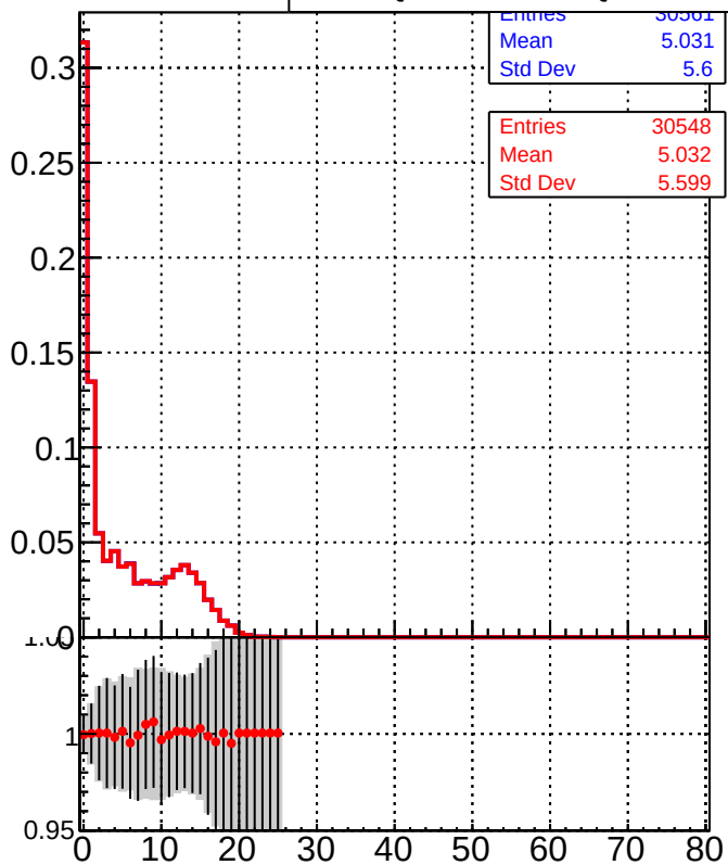
Legend: QDM_TT_mkFit-QDM_init_orig (grey vertical bars) QDM_TT_mkFit-QDM_init_modi2 (red line with diamonds)
