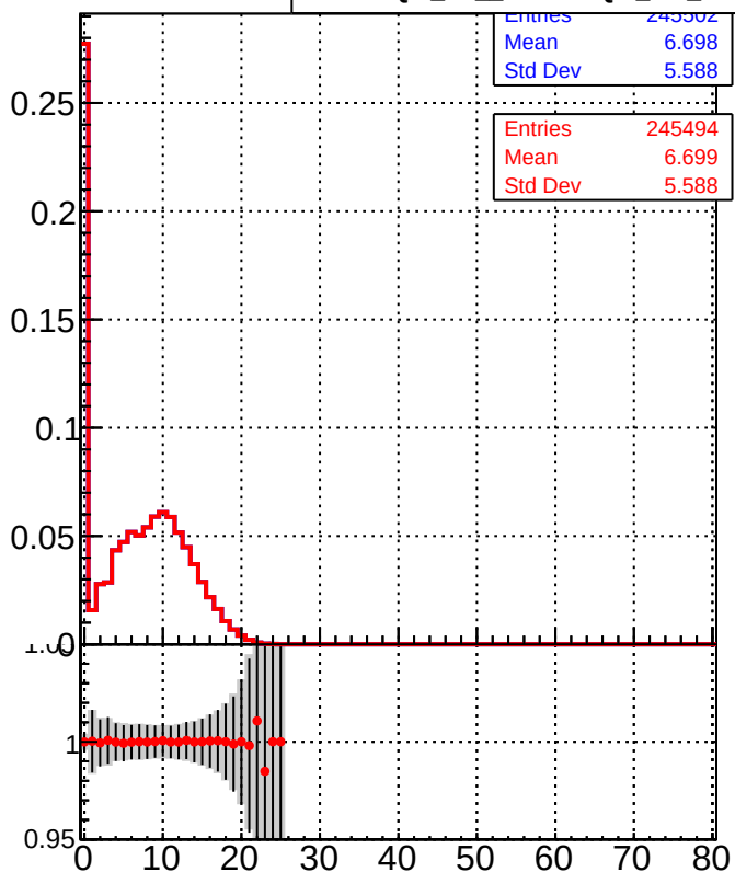
Legend: DQM_TT_mkFit-DQM_init_orig DQM_TT_mkFit-DQM_init_modi2
