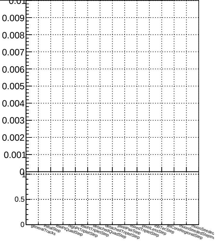
Duplicates rate vs collection Legend: DQM_TT_mkFit-DQM_init_orig (Blue square) DQM_TT_mkFit-DQM_init_modi2 (Red circle)
