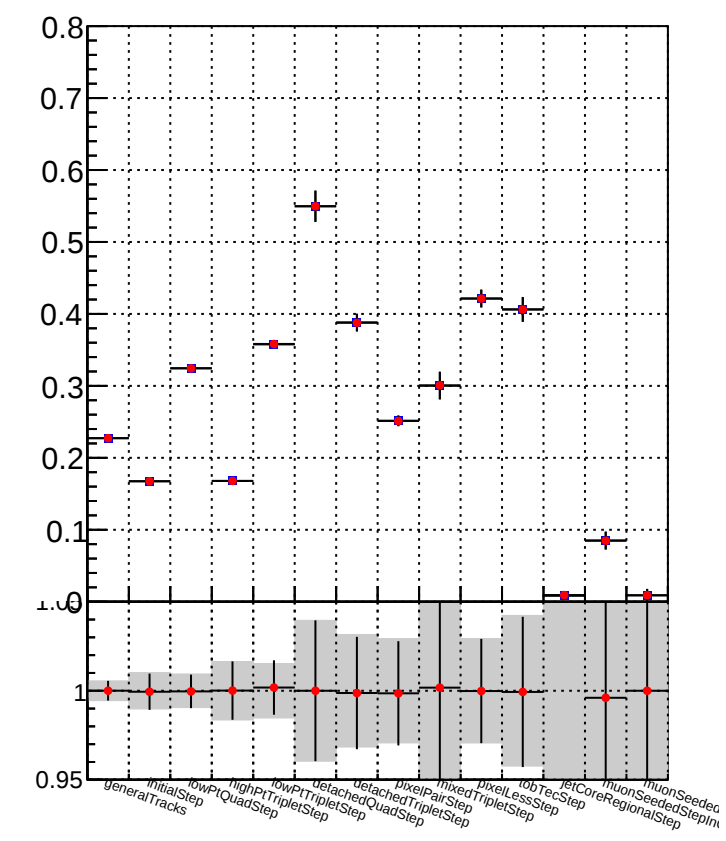
Duplicates rate vs collection Legend: DQM_TT_mkFit-DQM_init_orig (Blue square) DQM_TT_mkFit-DQM_init_modi2 (Red circle)
