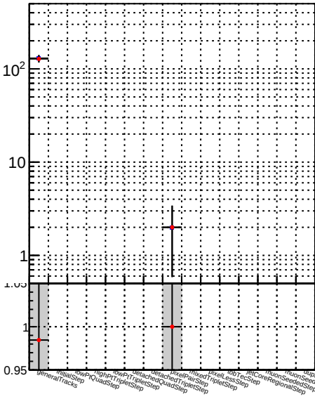
Number —●— DQM_TT_mkFit-DQM_init_modi2
