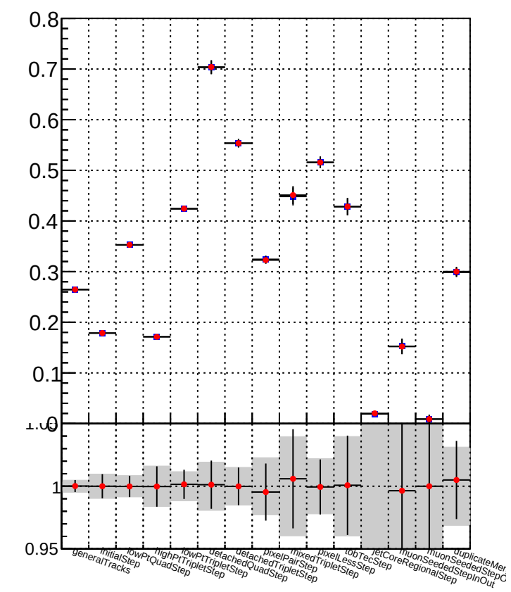
Duplicates rate vs collection Legend: ■ DQM_TT_mkFit-DQM_init_orig ● DQM_TT_mkFit-DQM_init_modi2
